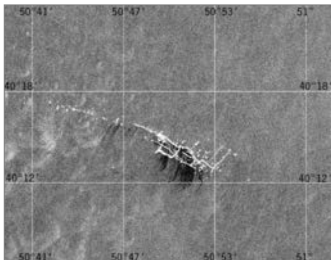
A subset of Sentinel-1A SAR image acquired at 02:44 UTC on 08.04.2020 showing the sea surface near the oil-drilling platform. A relatively small area of 12 sq. km covered by oily films can be identified near the oil-drilling platform
