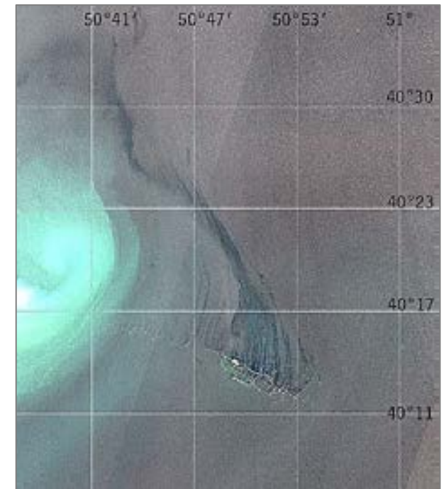
A subset of a true-colour MSI Sentinel-2B image (composite of 4, 3 and 2 spectral channels) acquired on 15 April 2020 outside the sunlint zone.
