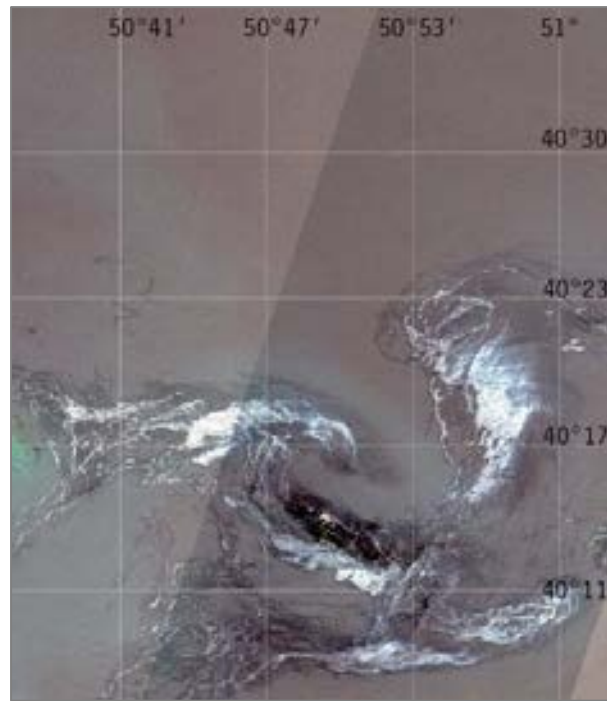
A subset of a true-colour MSI Sentinel-2B image (composite of 4, 3 and 2 spectral channels) acquired on 4 July 2020 in the sunlint zone
