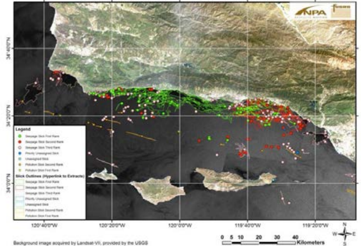
Oil slicks mapped from satellite SAR, Santa Barbara
