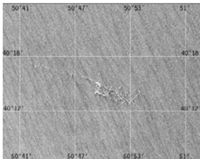
A subset of Sentinel-1A SAR image acquired at 14:29 UTC on 16.03.2020 over the oil-producing area Oil Rocks
