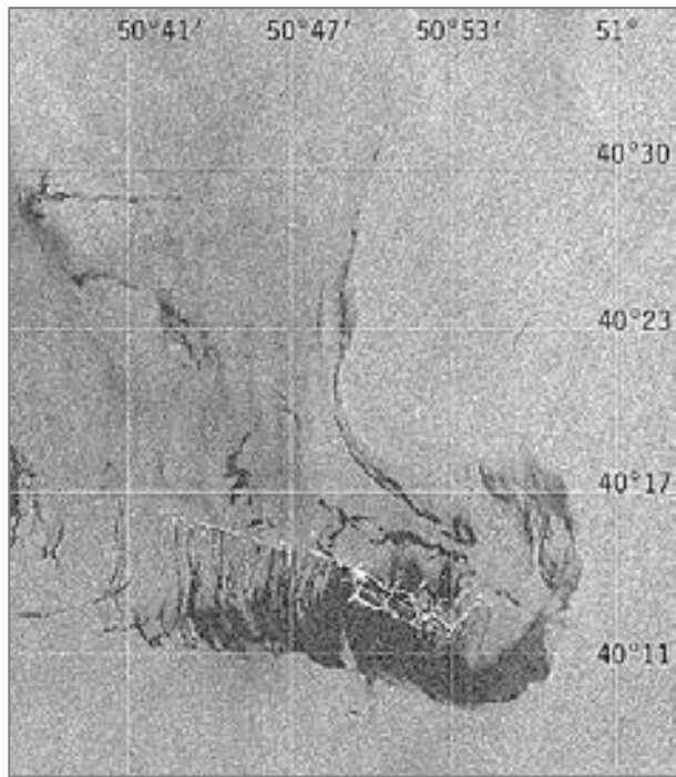
A subset of a Sentinel-1A image acquired on 2 February 2019
