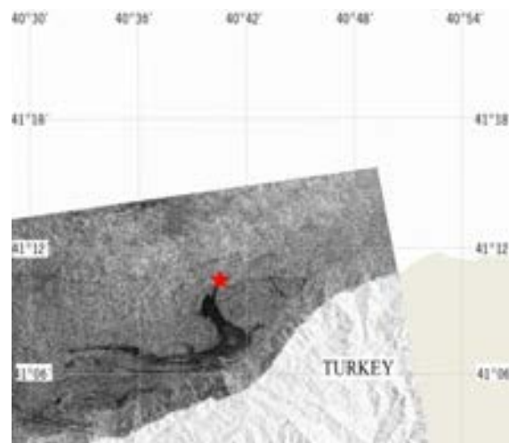
Examples of natural oil slicks in satellite radar images of the southeast Black Sea: a) Sentinel-1A SAR, 24.06.2015, 15:10 UTC; b) Sentinel-1A SAR, 01.03.2015, 15:18 UTC; c) Sentinel-1A SAR, 19.02.2016, 15:10 UTC; d) Sentinel-1A SAR, 14.12.2015, 15:18 UTC. Asterisks mark the oil slicks origin location.
