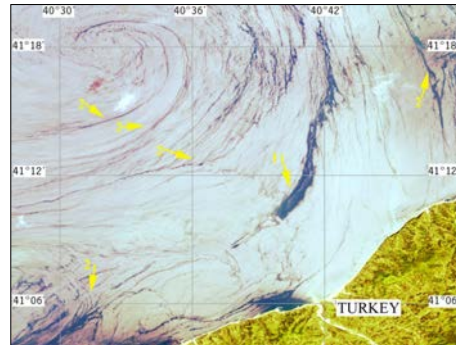
A part of a Landsat-8 OLI image (composite of 4, 3 and 2 spectral channels) of 29 May 2014, 08:01 UTC.
