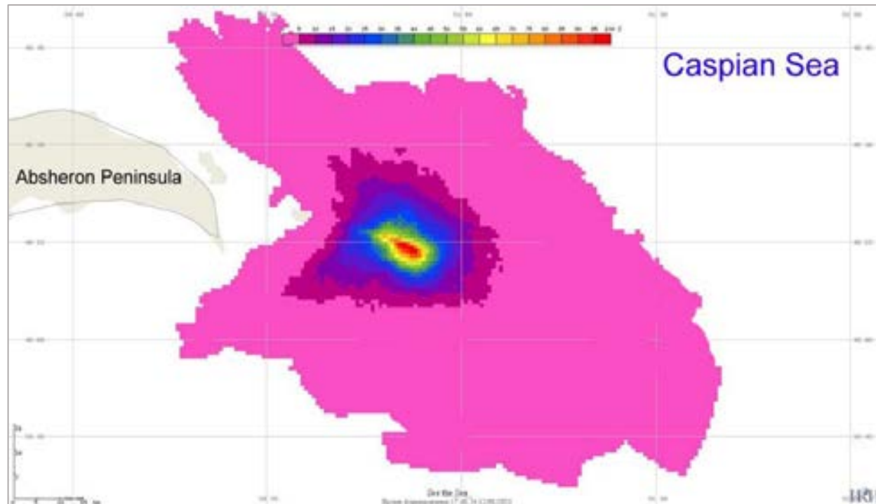
The probability of the pollution by crude oil of the sea surface near the Oil Rocks oil-producing site calculated based on satellite data
