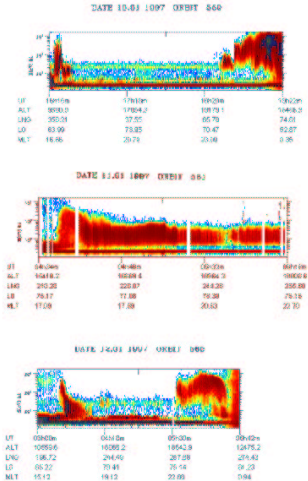
Fig. 10. The electron energy spectrograms during 3 orbits of INTERBALL-2 on January 10-12, 1997.
