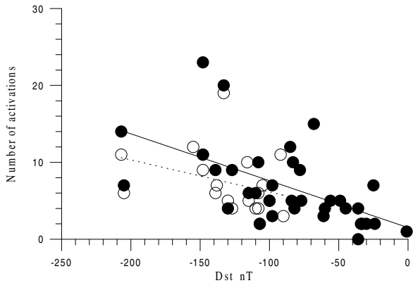
Fig. 6. Observed values of the number of activations NA and minimum of D_{st} for magnetic cloud (black circles) and strong magnetic storms (white circles) periods.
