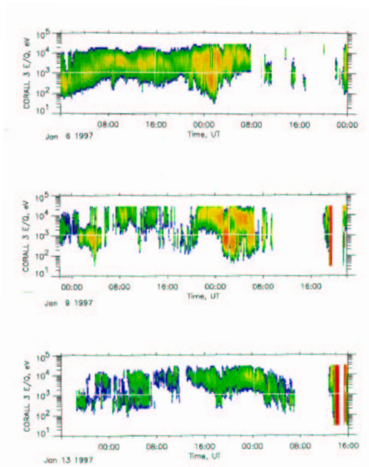
Fig. 9. The ion energy spectrograms during 3 successive orbits of INTERBALL-1 on January 6-15, 1997.
