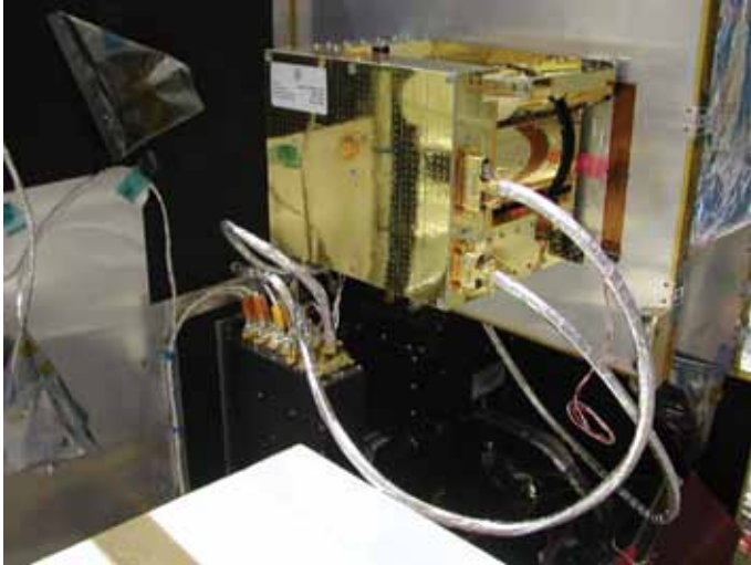
Figure 3. PFS for Mars Express integrated on the spacecraft: visible are Module P (Power Supply), Module E (digital electronics), Module S (the rotating mirror), Module O (Interferometer with proximity electronics) is inside the spacecraft structure.
