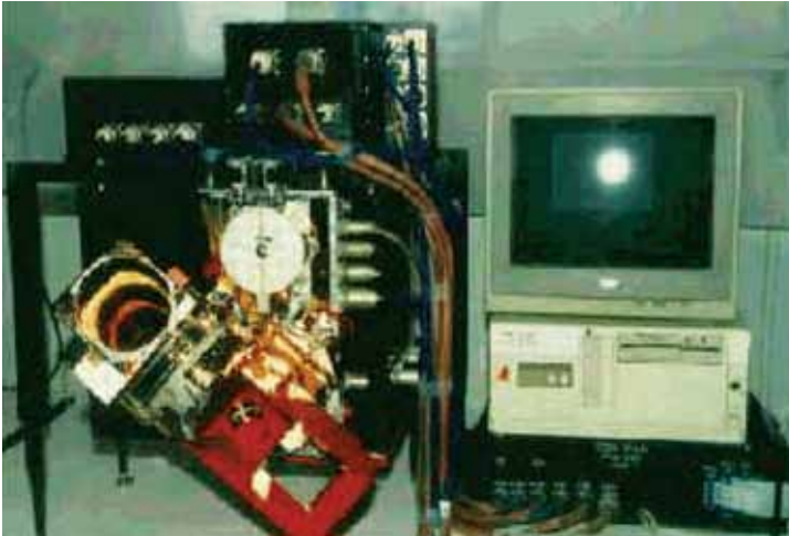
Figure 2. Functionality test of PFS for Mars 96 in Frascati, 1994. The scanner had two degrees of freedom (two rotation axis). Cables and connectors were Russian provided. The boxes were: Module O, Power supply, Digital electronics, Pointing device, Controller of Pointing device. Visible are also: GSE interface (black) and controlling computer.
