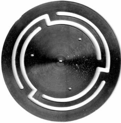
Figure 1. Scheme of the aluminium membrane to hold the moving mirror for a Michelson concept PFS (1990). Not implemented later.
